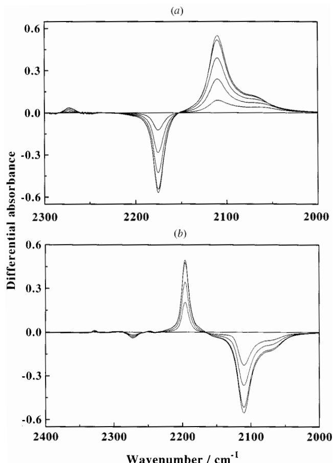
Fig. 2 Changes in IR difference absorption spectra accompanying (a) reduction of \text{trans}[\text{RuBr}_4(\text{CNBu}^t)_2]^- in 0.25 \text{ mol dm}^{-3} [\text{NBu}_4][\text{PF}_6] in acetonitrile–dichloromethane (1 : 1) in an IRRAS cell at room temperature. The horizontal line at zero absorbance corresponds to the initial spectrum, i.e. that of \text{trans}[\text{RuBr}_4(\text{CNBu}^t)_2]^- , prior to electrolysis. The potential of the working electrode is stepped to E_{\text{app}} = -0.4 \text{ V} , and single-scan IR spectra collected as a function of time. Consumption of \text{trans}[\text{RuBr}_4(\text{CNBu}^t)_2]^- , upon reduction, is indicated by increasing negative absorbance at 2170 \text{ cm}^{-1} , whilst increasing positive absorbance at 2272 and 2109 \text{ cm}^{-1} corresponds to the formation of \text{mer,trans}[\text{RuBr}_3(\text{CNBu}^t)_2(\text{NCMe})]^- ; (b) oxidation of \text{mer,trans}[\text{RuBr}_3(\text{CNBu}^t)_2(\text{NCMe})]^- to \text{mer,trans}[\text{RuBr}_3(\text{CNBu}^t)_2(\text{NCMe})] at E_{\text{app}} = +0.6 \text{ V}
