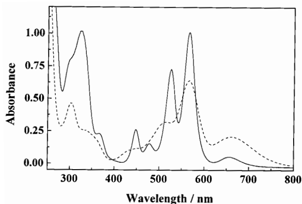
Fig. 3 The UV/VIS spectra of \text{trans}[\text{RuBr}_4(\text{CNBu}^t)_2]^- (—) and \text{mer,trans}[\text{RuBr}_3(\text{CNBu}^t)_2(\text{NCMe})] (---), recorded in an OTTE cell at 243 \text{ K} , in 0.25 \text{ mol dm}^{-3} [\text{NBu}_4][\text{PF}_6] in acetonitrile–dichloromethane (1 : 1)
